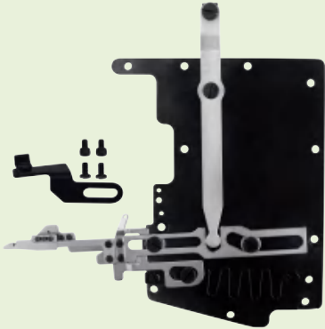
刀盘 Knife Carrier
