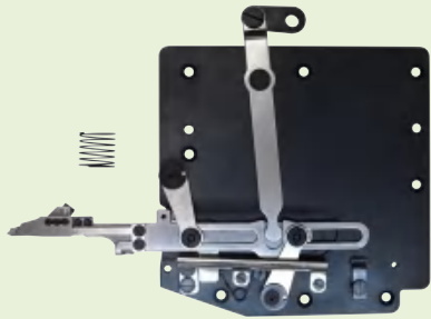
刀盘 Knife Carrier
