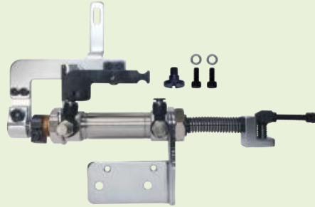
气动下剪线组件 Air Under Trimmer Drive
