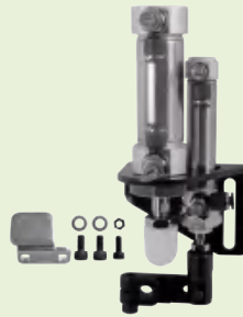
抬压脚组件 Presser Foot Lifter
