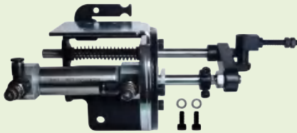
气动下剪线组件 Air Under Trimmer Drive
