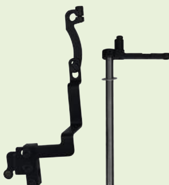
松线传动组件 Transmission Unit of Tension Disc Separator
