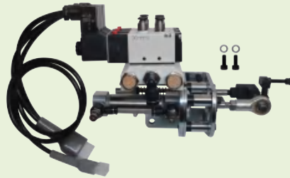
气动下剪线组件 Air Under Trimmer Drive
