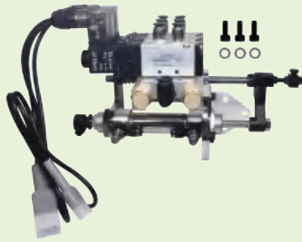
气动下剪线组件 Air Under Trimmer Drive
